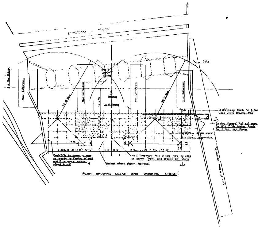
Fig. 275.—Arrangement of Plant with Working Stage.
